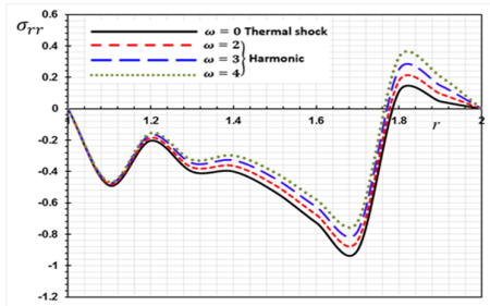
Figure 8. The effect of thermal vibration \omega on the radial stress \sigma_{rr} .
