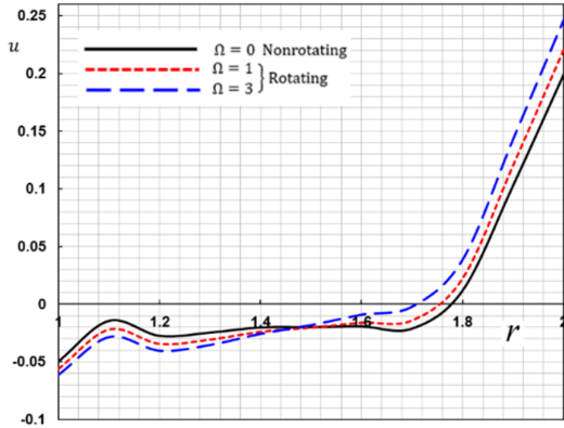
Figure 3. The effect of rotation \Omega on the displacement u .
