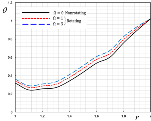
Figure 2. The effect of rotation \Omega on the temperature \theta
