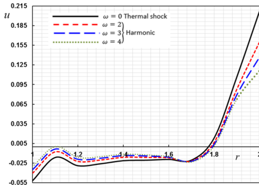
Figure 7. The effect of thermal vibration \omega on the displacement u .
