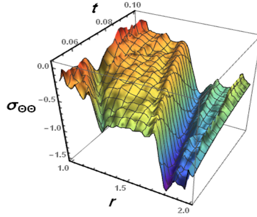
Figure 13. The hoop stress \sigma_{\theta\theta} with different time.
