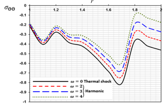
Figure 9. The effect of thermal vibration \omega on the hoop stress \sigma_{\theta\theta} .
