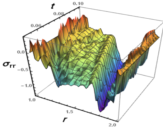
Figure 12. The radial stress \sigma_{rr} with different time.
