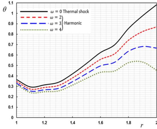
Figure 6. The effect of thermal vibration \omega on the temperature \theta .
