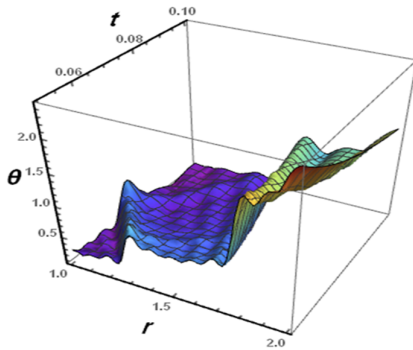
Figure 10. The temperature \theta with different time.
